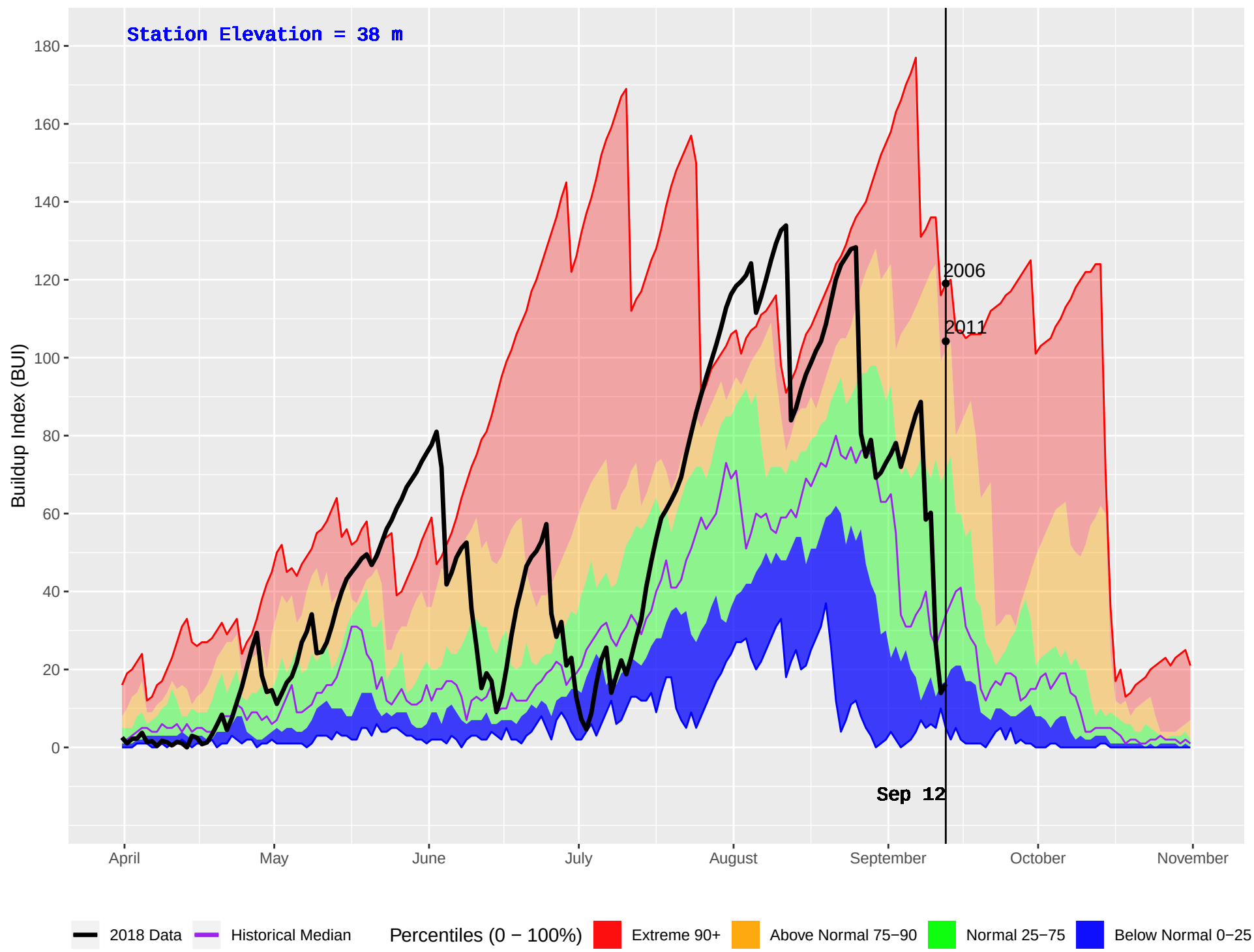
HAIG CAMP (67) : Historical (2002–2016) and Current (2018) Daily Buildup Index (BUI)
