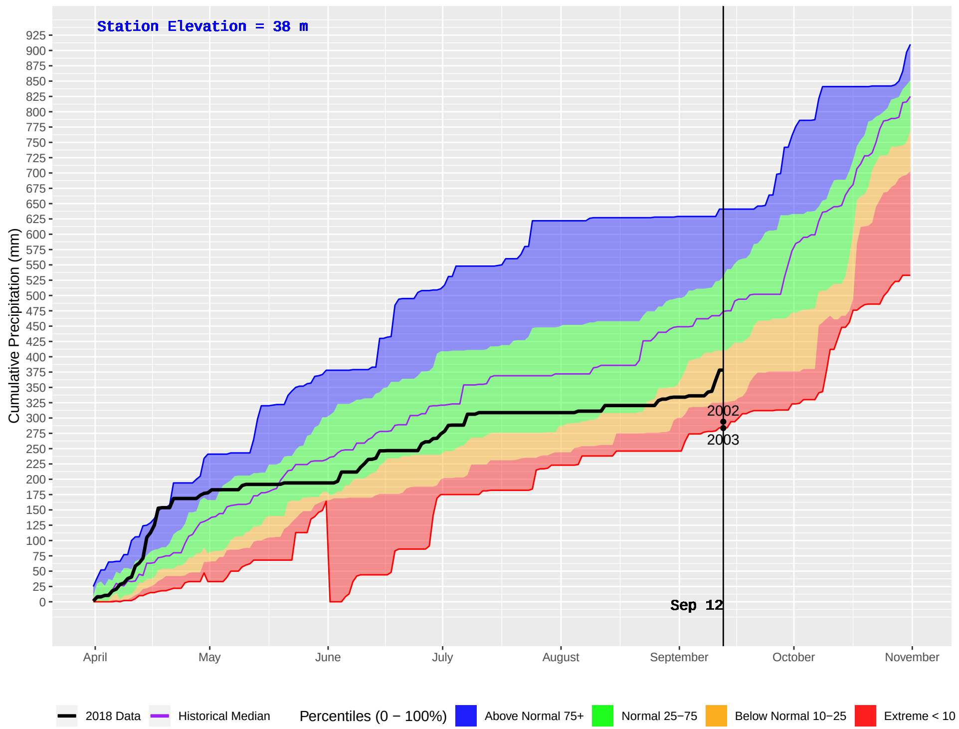
HAIG CAMP (67) : Historical (2002–2016) and Current (2018) Daily Cumulative Precipitation
