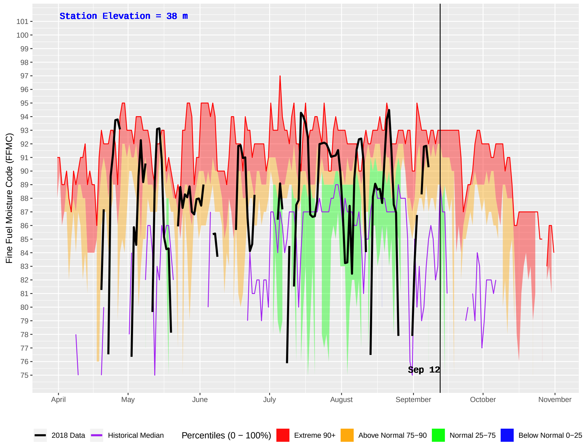
HAIG CAMP (67) : Historical (2002–2016) and Current (2018) Daily Fine Fuel Moisture Code (FFMC)
