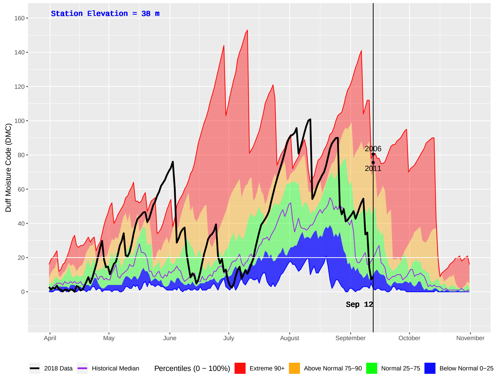
HAIG CAMP (67) : Historical (2002–2016) and Current (2018) Daily Duff Moisture Code (DMC)
